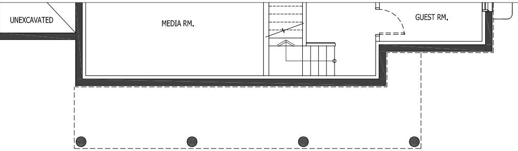
LOWER LEVEL | ELEVATION B 820 sq. ft.
