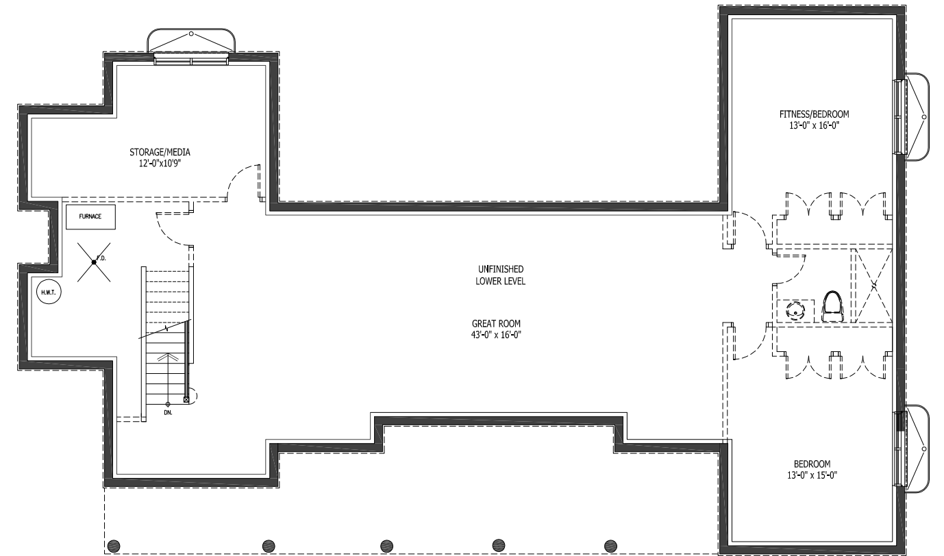
LOWER LEVEL 1,551 sq. ft.
