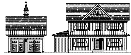
ELEV. A | without finished coach house
