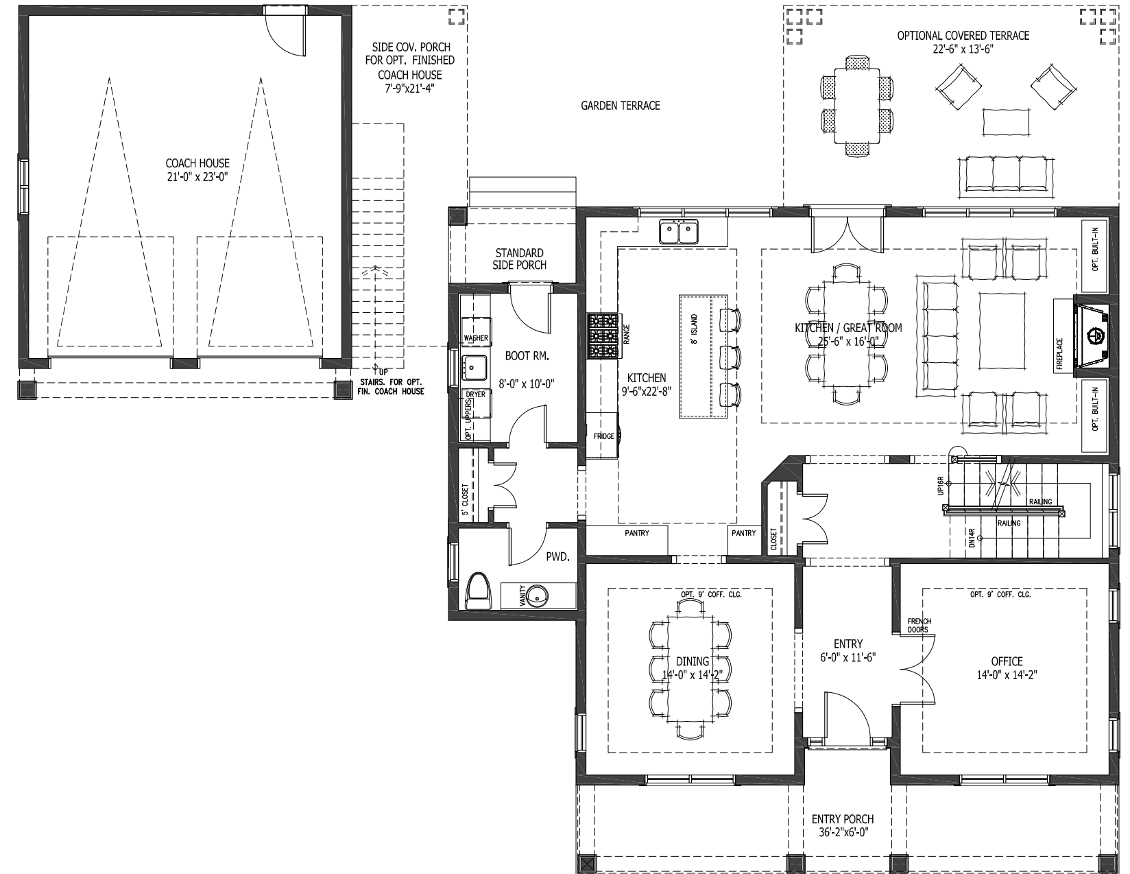
MAIN LEVEL 1,590 sq. ft.
