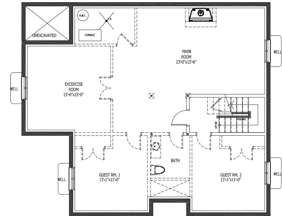
LOWER LEVEL 1,248 sq. ft. (34 sq. ft. finished lower foyer)
