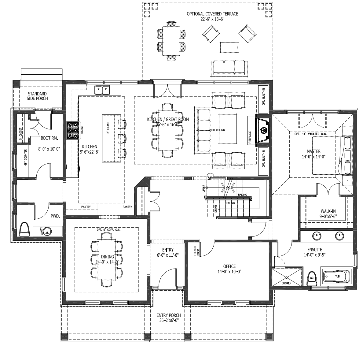
MAIN LEVEL 2,042 sq. ft.
